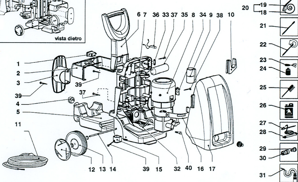
Exploded drawing E8062C001/01
